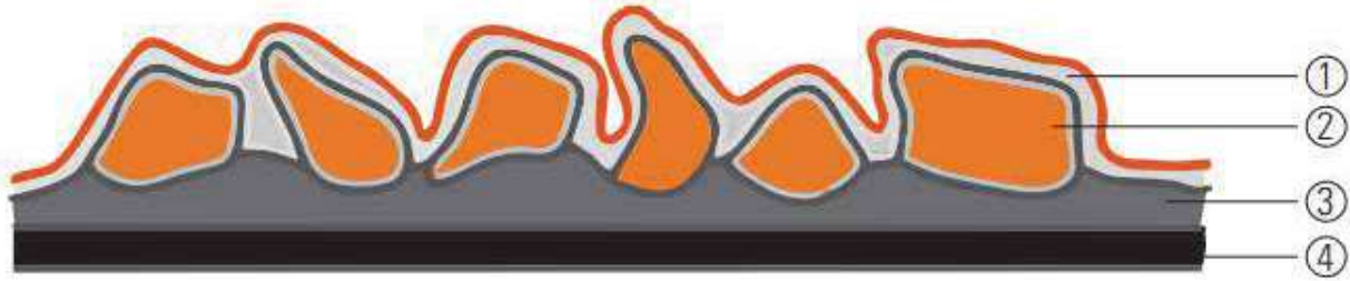
1. Size Coat 2. Mineral Grit 3. Glue or Resin Bond 4. Backing
